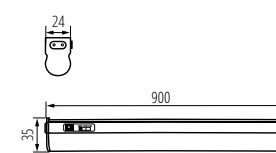
NERA LED 11W CCT
