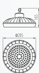
HB PRO LED HI 100W
